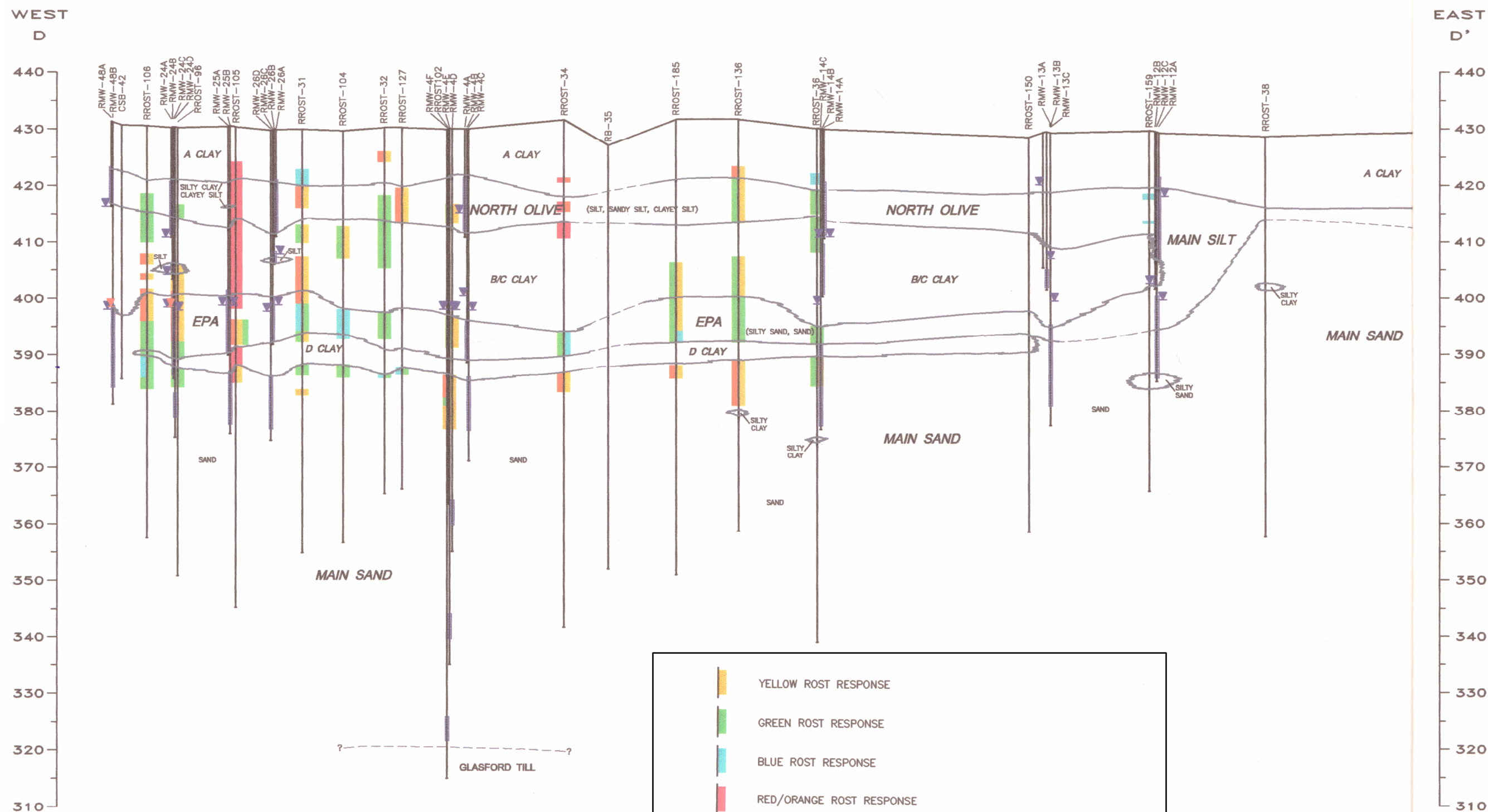
HARTFORD AREA HYDROCARBON PLUME SITE HARTFORD, ILLINOIS FIGURE 11 CROSS-SECTION D-D' THROUGH WASTEWATER TREATMENT PLANT AND NORTH BULK TANK STORAGE AREA
