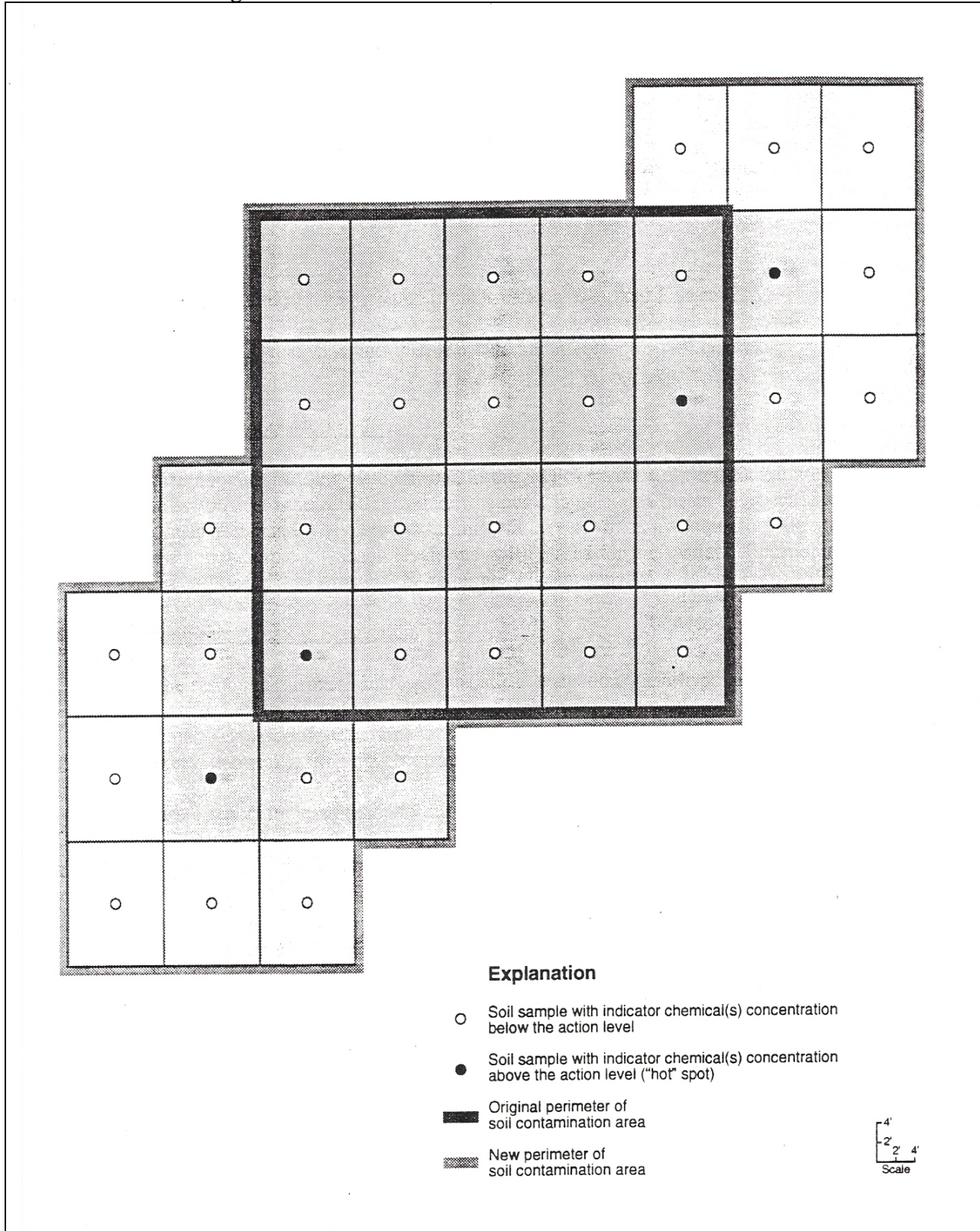
Figure 3. Definition of Lateral Extent of Excavation
