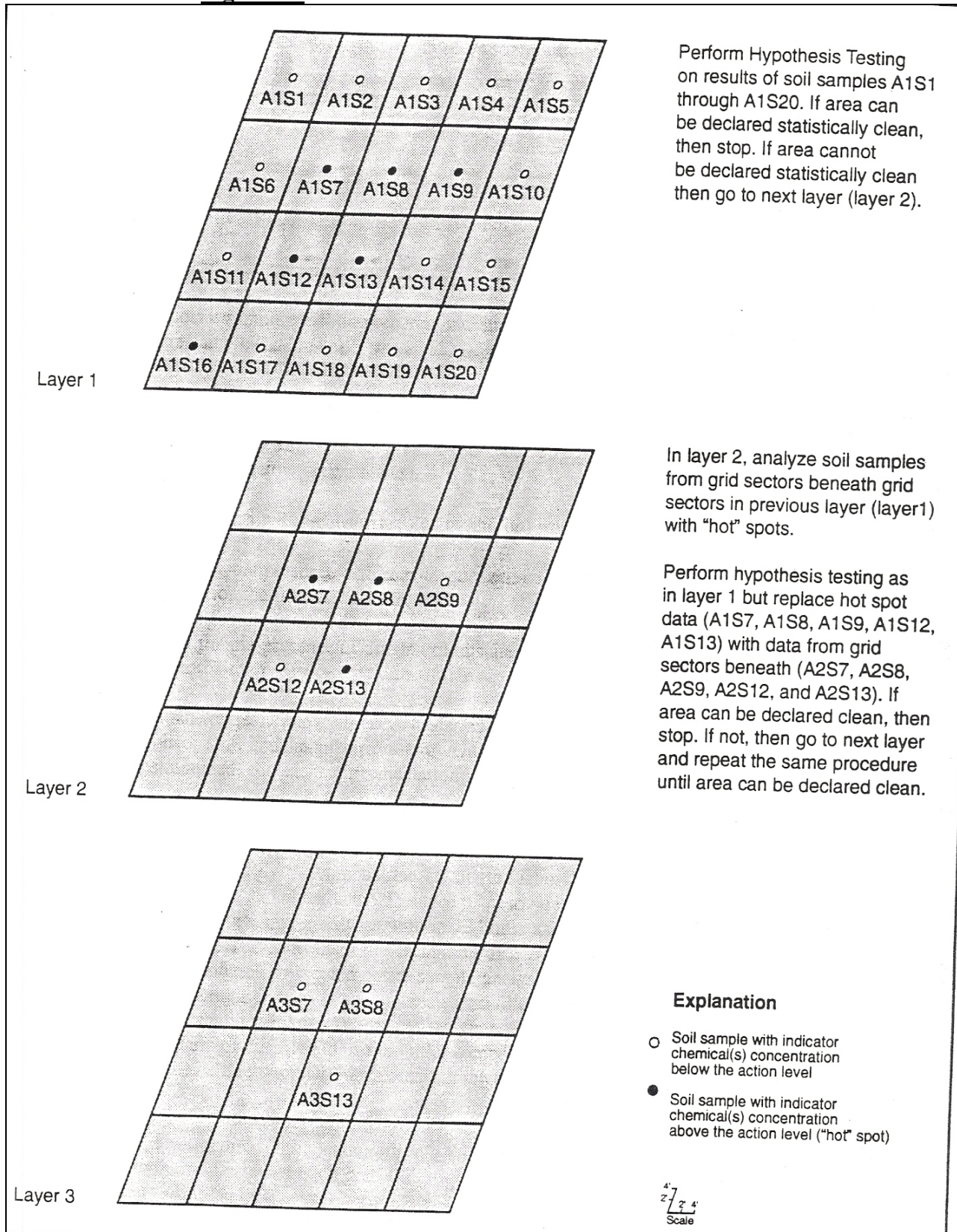
Figure 4. Definition of Vertical Extent of Excavation
